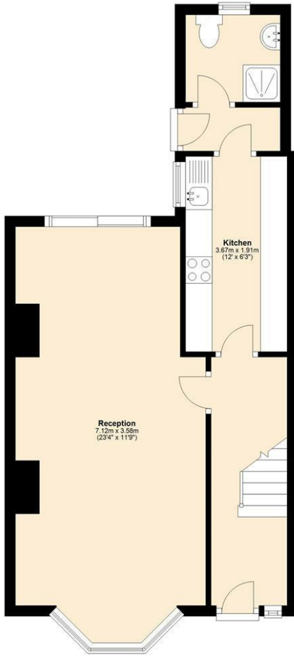
Ground Floor Approx. 44.0 sq. metres (473.2 sq. feet)
